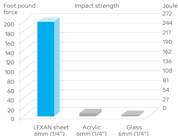
FIGURE 1 IMPACT RESISTANCE Falling dart impact test 5 pounds (2.3 kg.) steel dart 1" (25.4 mm) diameter dip
