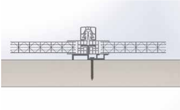
Snap batten onto standing seam
